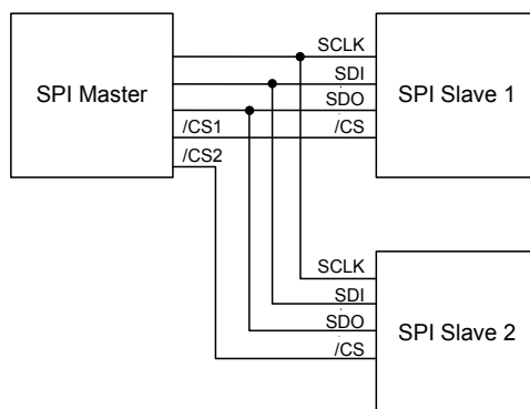
Typical SPI Master / Slave Configuration
